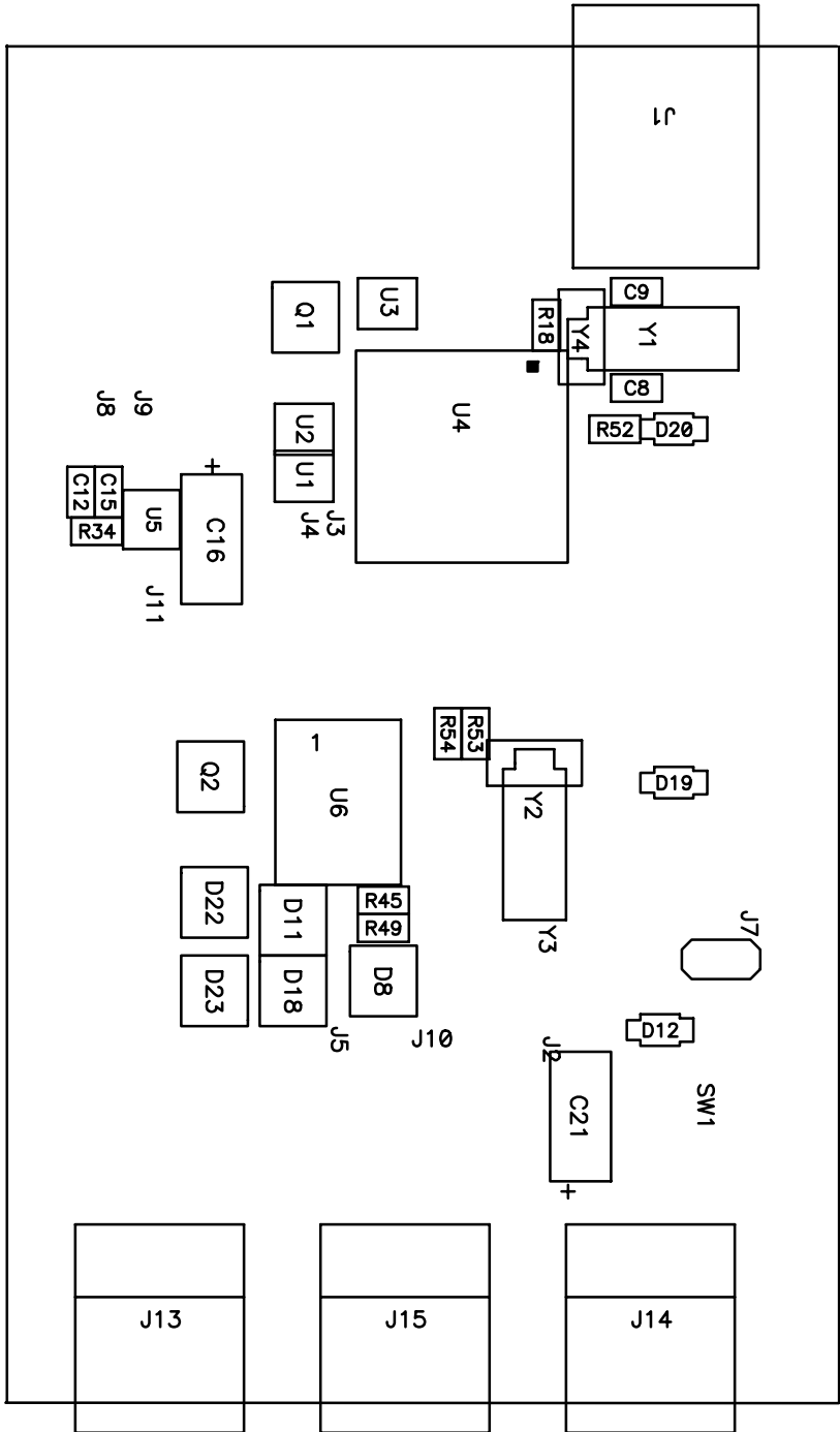
Figure 3-5. Component Placement 1
