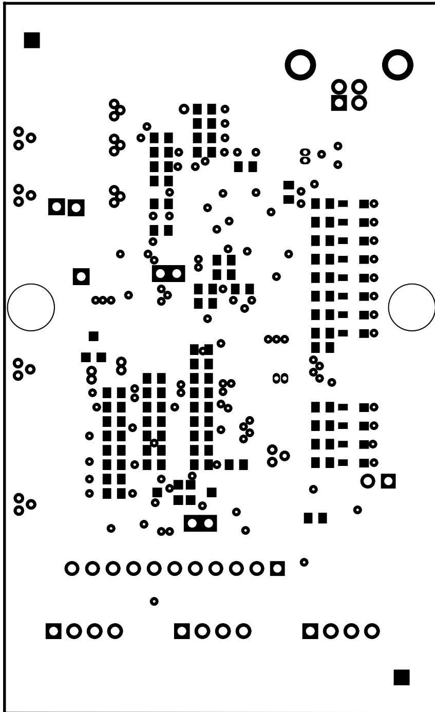
Figure 3-3. Solder Mask 2
